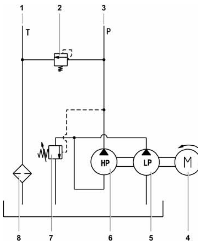
Flow chart for hydraulic aggregate
